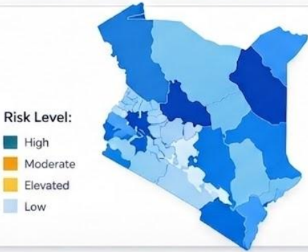
Kenya Risk Map
